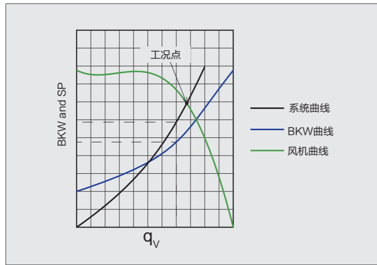
Fig.4 Operating Point
