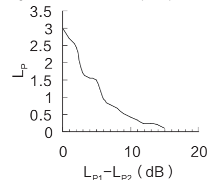
图 1 两噪声源的叠加曲线 Fig 1. Two noise sources superimposed curve
